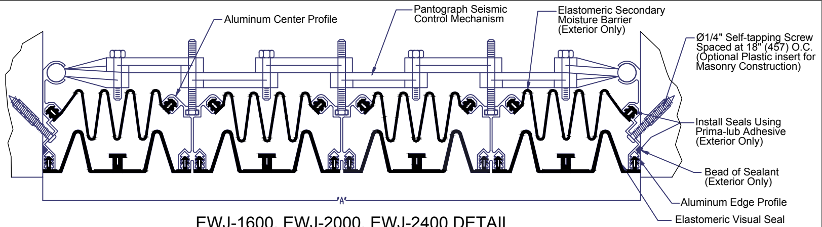
EWJ-1600, EWJ-2000, EWJ-2400 DETAIL EXTERIOR APPLICATION / WALL TO WALL
