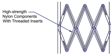
PLAN VIEW PANTOGRAPH CONTROL MECHANISM
