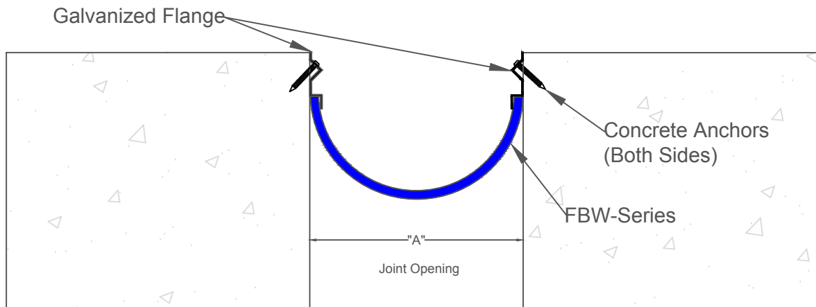
FBW-Series Wall to Wall Condition
