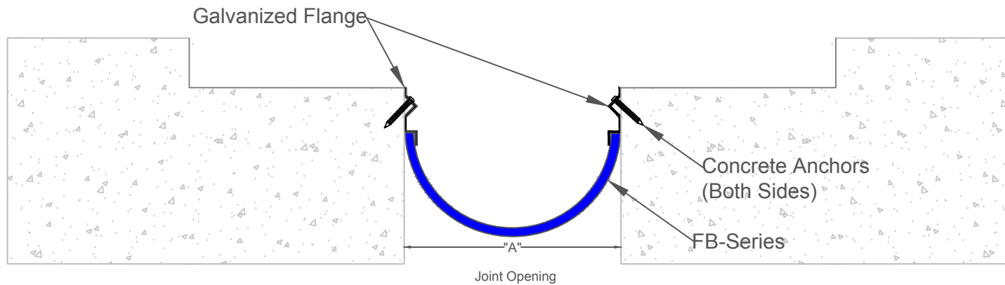
FB-Series Floor to Floor Condition
