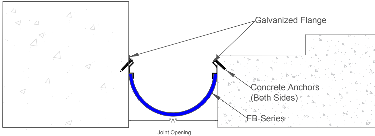
FB-Series Floor to Wall Condition
