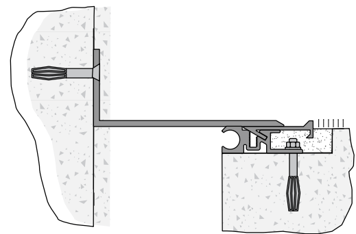
Floor-to-Wall/Corner
