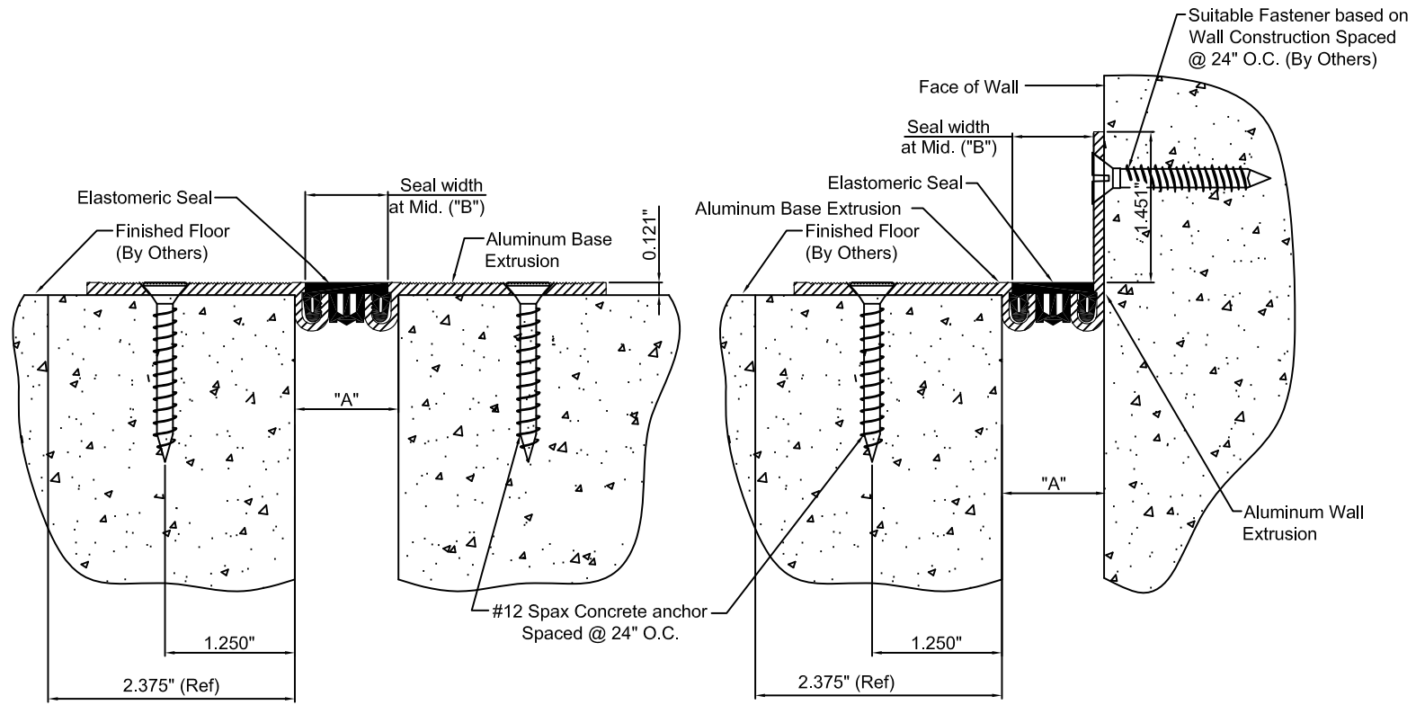
ELCFT-100 DETAIL FLOOR TO FLOOR CONDITION
