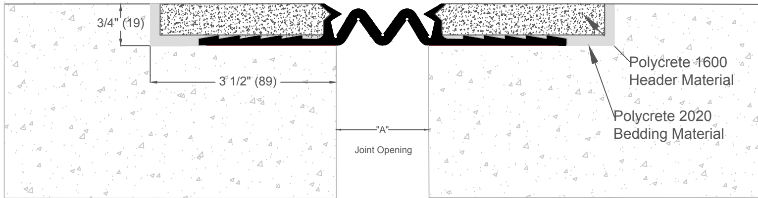
WM-SERIES Slab to Slab Condition
