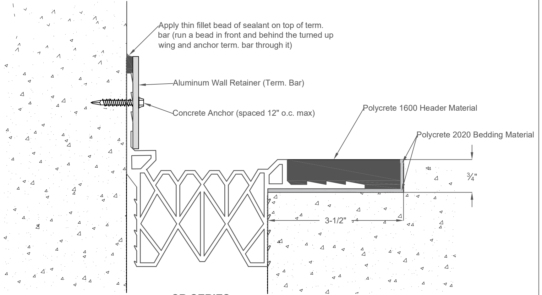
CR-SERIES Slab to Wall Condition
