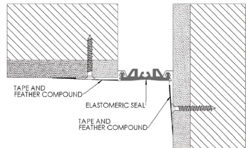
WALL-TO-WALL/CORNER
