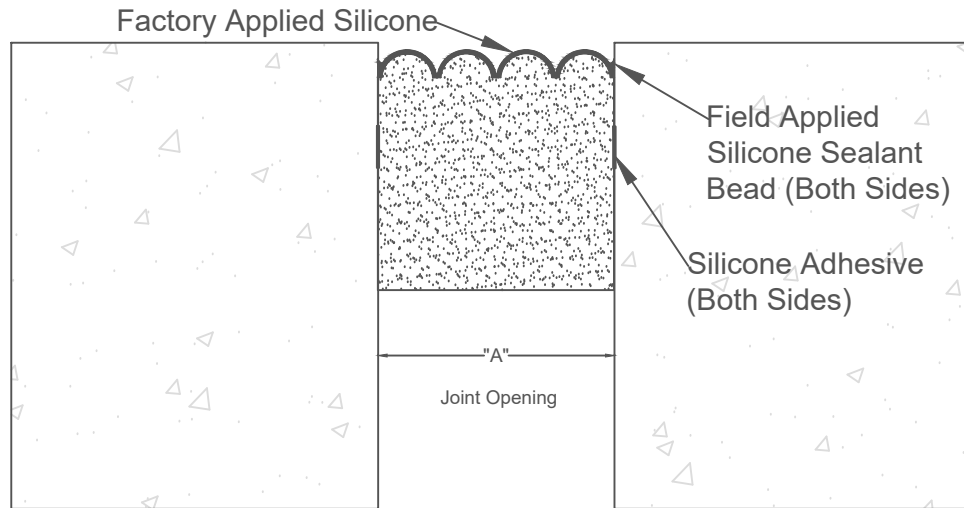
CSS-SERIES Vertical Condition
