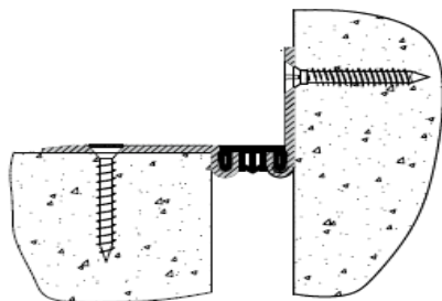
Floor-to-Wall/Corner
