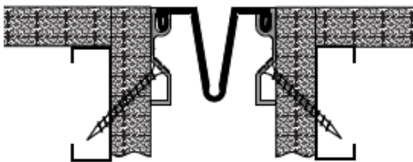
Wall/Ceiling Corner
