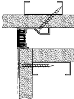
Wall/Ceiling Corner
