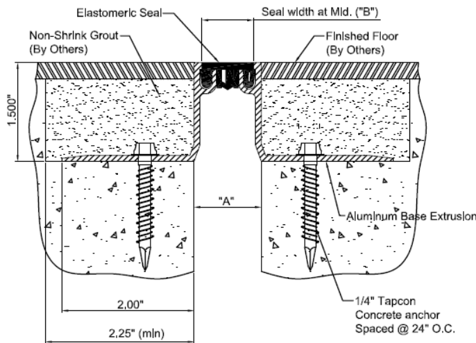
ELCF-100 DETAILS FLOOR TO FLOOR CONDITION
