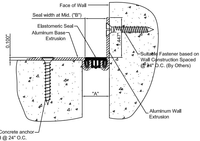
ELCFS-100W DETAIL FLOOR TO WALL CONDITION
