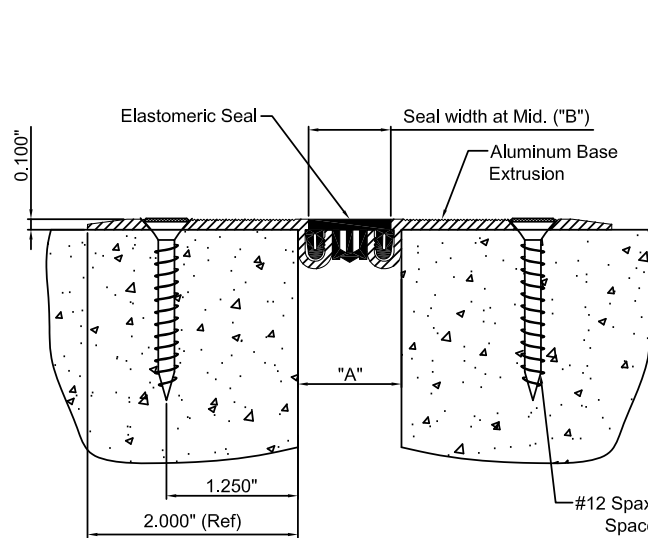
ELCFS-100 DETAIL FLOOR TO FLOOR CONDITION
