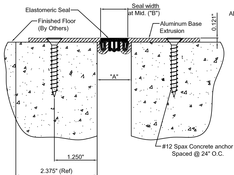
ELCFT-100 DETAIL FLOOR TO FLOOR CONDITION
