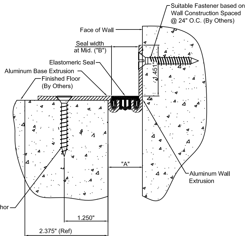
ELCFT-100W DETAIL FLOOR TO WALL CONDITION
